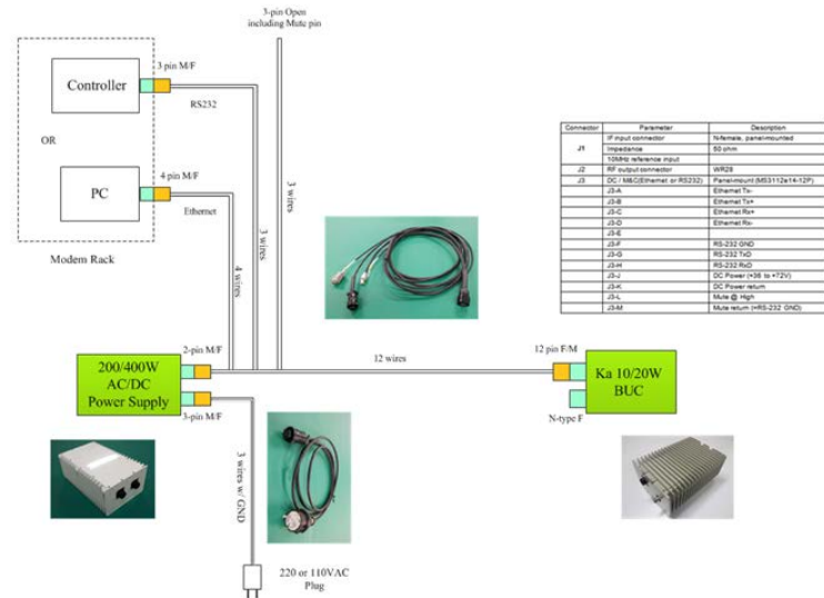
Ka 10/20W BUC + Power Supply + Cable Assembly Configuration
